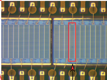
SiPM channel 250\mu\text{m} \times 1625\mu\text{m}
