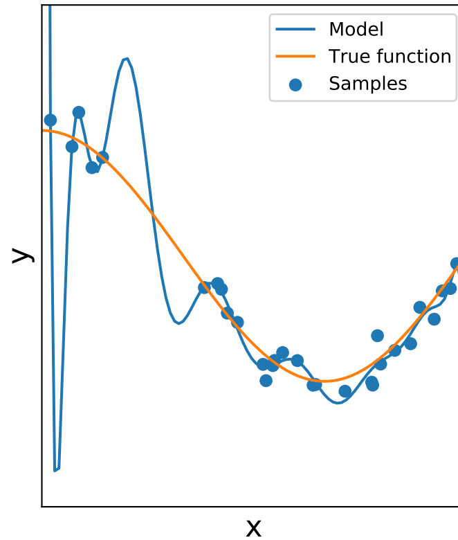
Degree 15 MSE = 1.80e+08 ( \pm 5.41e+08 )
