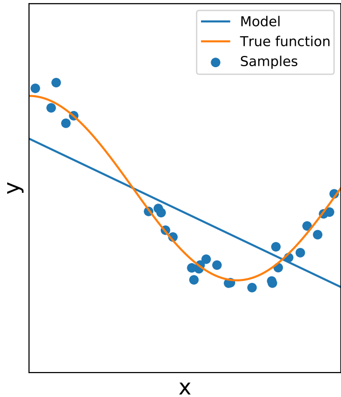
Degree 1 MSE = 4.08e-01 ( \pm 4.25e-01 )
