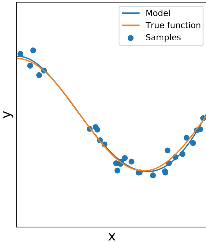
Degree 4 MSE = 4.32e-02 ( \pm 7.08e-02 )
