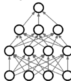
Original Network
